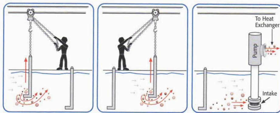
Figure 1. Cleaning traditional single or double fixed-grate screens can generate debris in downstream equipment. The absence of a pressure drop below the screen as it is lifted creates a reverse-eddy effect that pulls debris from the first screen into the second screen or suction pit (left). With double fixed-grate screens, the debris is stirred up when the second screen is removed for cleaning or periodic maintenance (center). Once the contaminants enter the suction pit, they are ground up by the pump and sent downstream to the heat exchangers (right).
