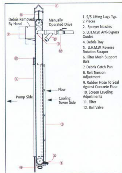
Figure 2. The traveling screen is designed to protect the process from any debris that might cause problems downstream.
